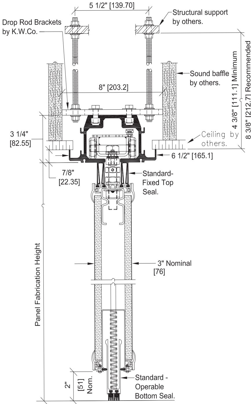
850 Curve & Diverter Aluminum Track and Carrier
