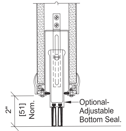
Optional Adjustable Bottom Seal
